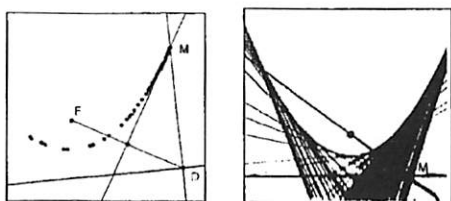
Fig.3. Multiple examples of constructing a parabola
